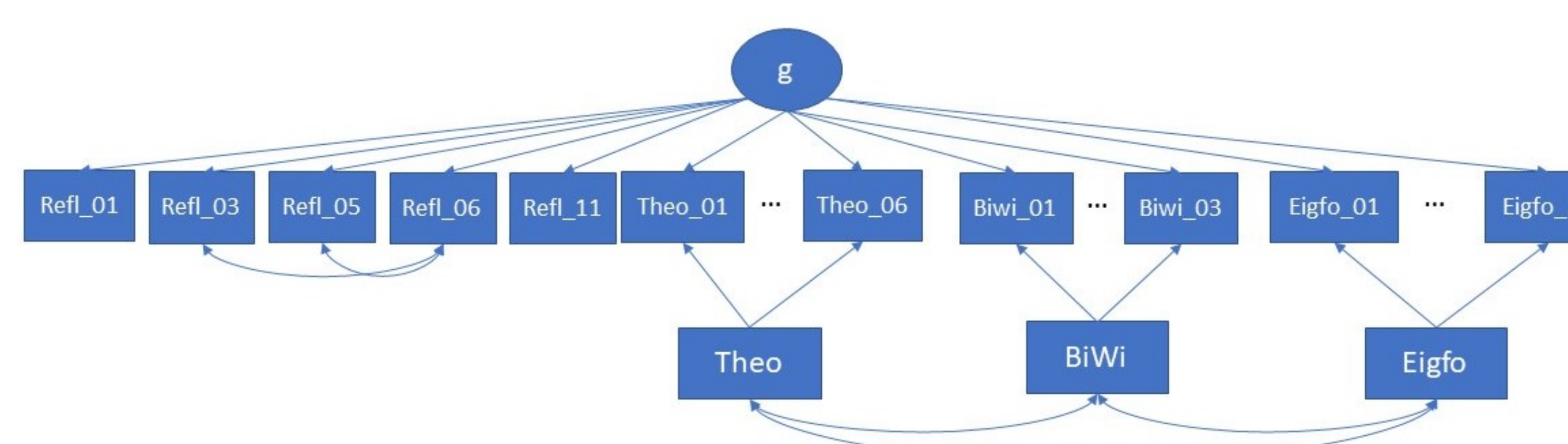
Figure 1: Bifactorial model of the overall structure of the instrument
